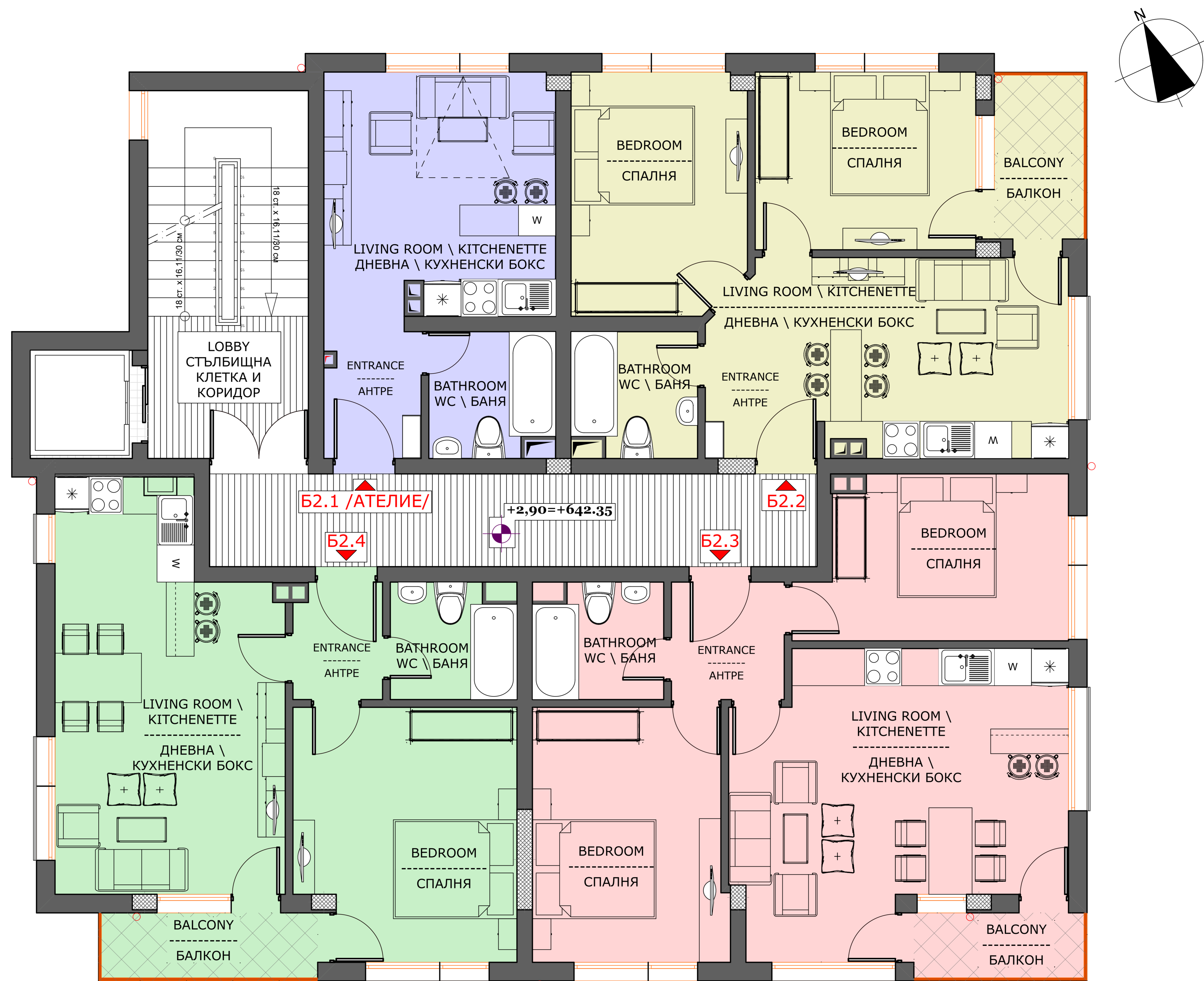
BUILDING - B level +2,90
