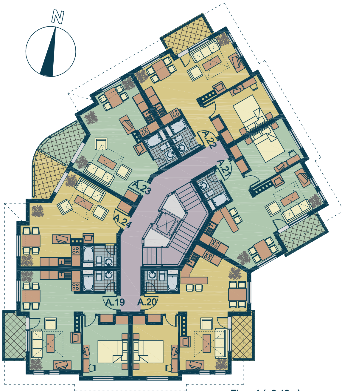
Floor 4 (+8,40m)
